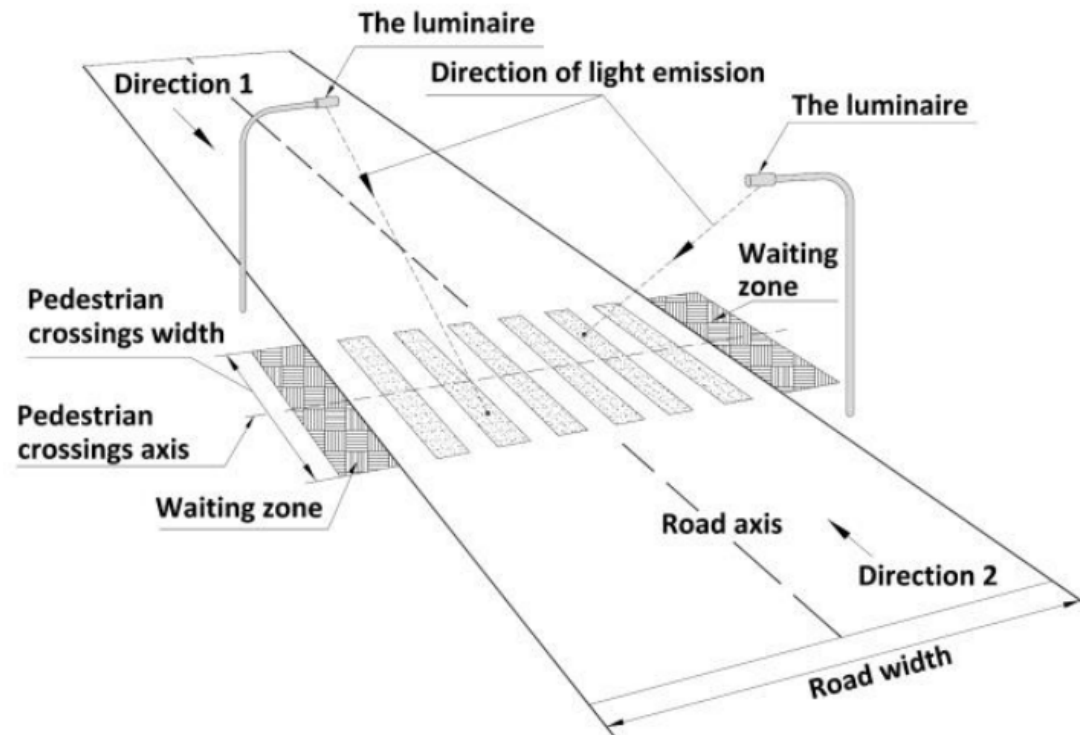
Fig. 7. Main directions of emission of dedicated luminaires.
