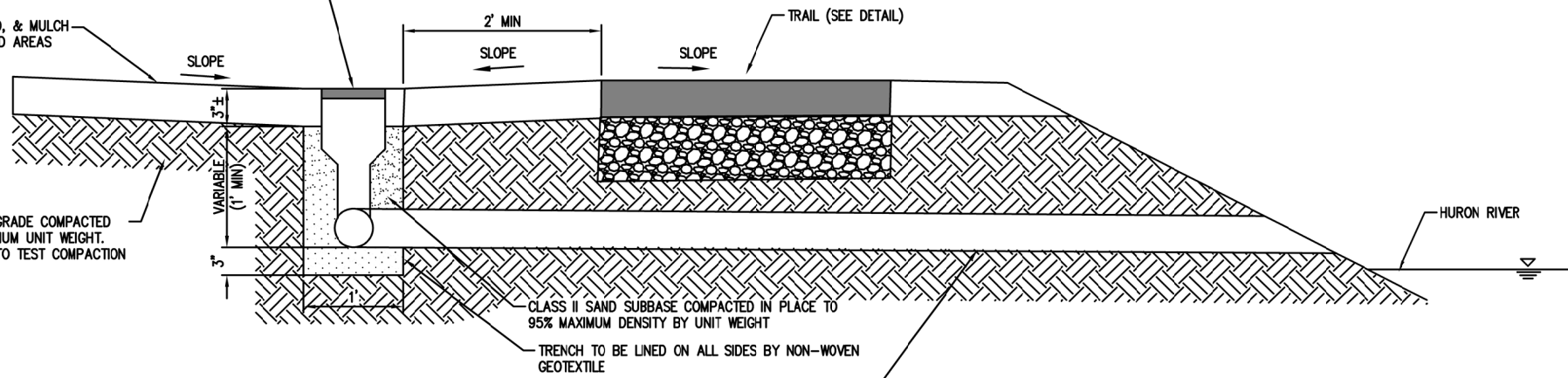
YARD DRAIN DETAIL NOT TO SCALE
