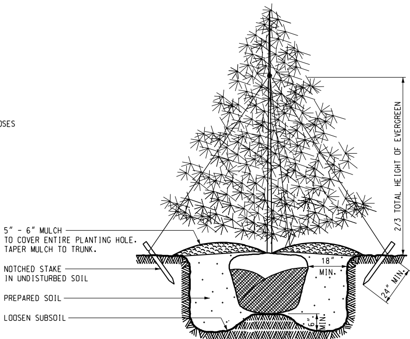
GUYING TRIPOD METHOD
