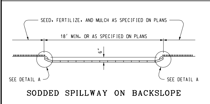
NORMAL SECTION WITH SODDED SPILLWAY DITCH
