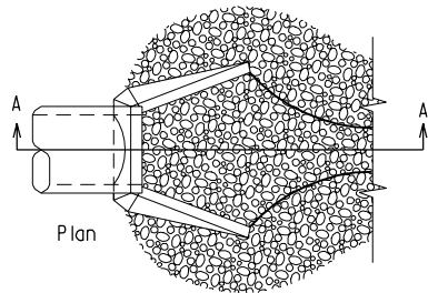
Pipe outlet to well-defined channel
