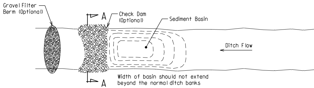
Plan View
