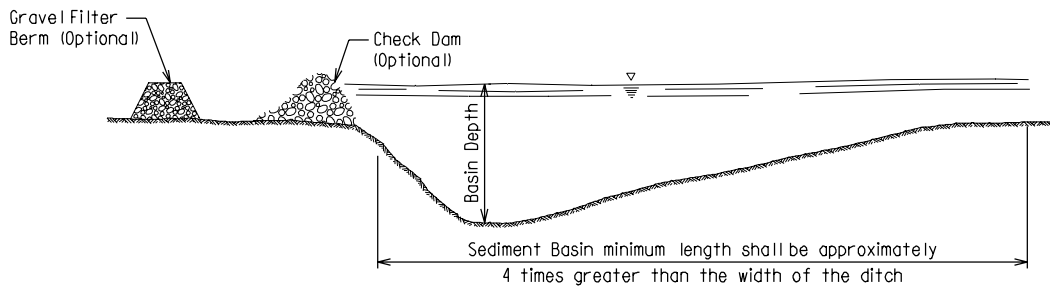
Profile View
