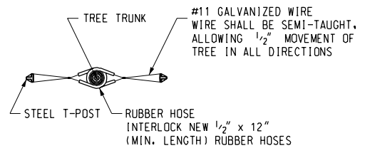
BRACING DETAIL
