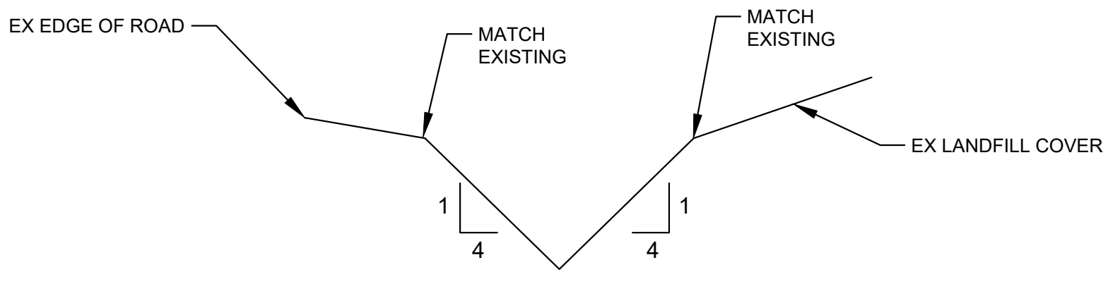
TYPICAL CROSS SECTION OF PROPOSED DRAIN
